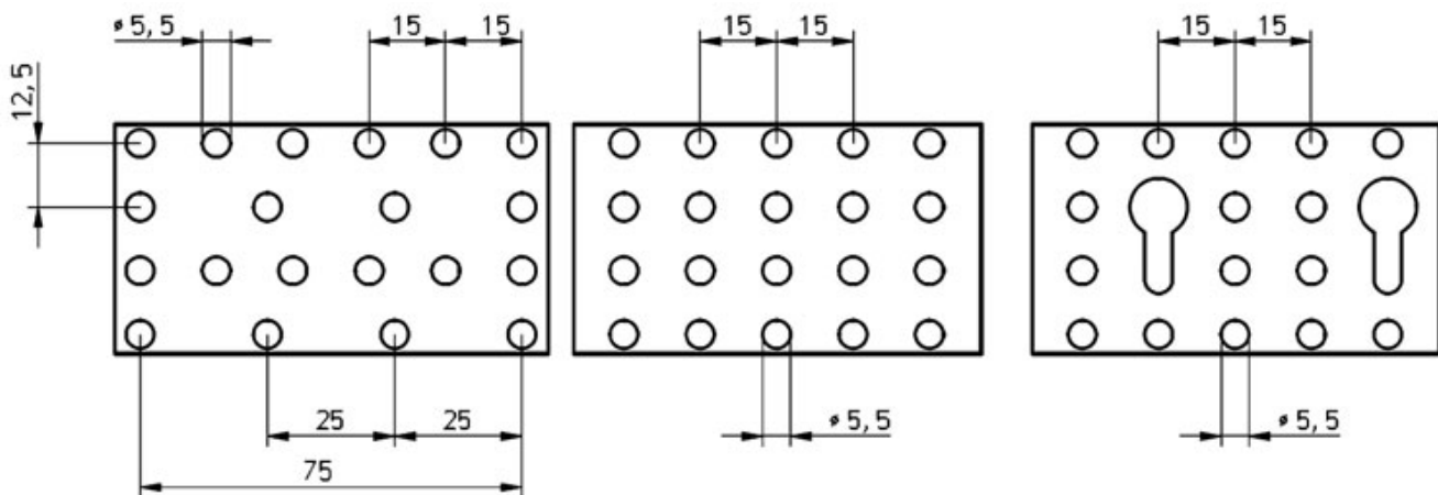
Eurolochung/Rundloch „Euro“-perforation/Round holes
